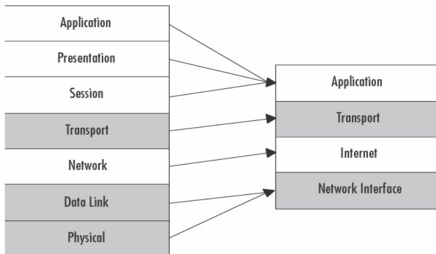
OSI Model
